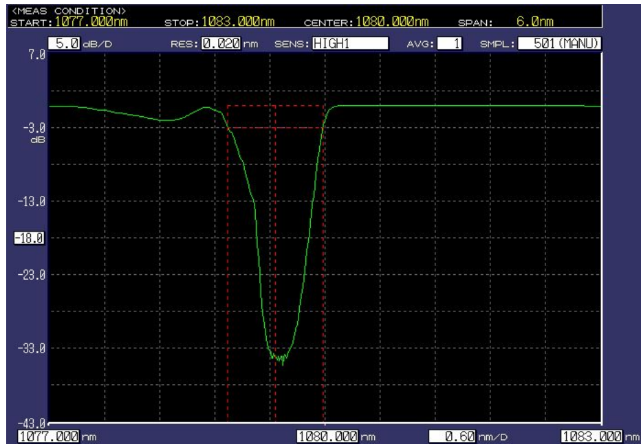
(Transmission spectrum)
